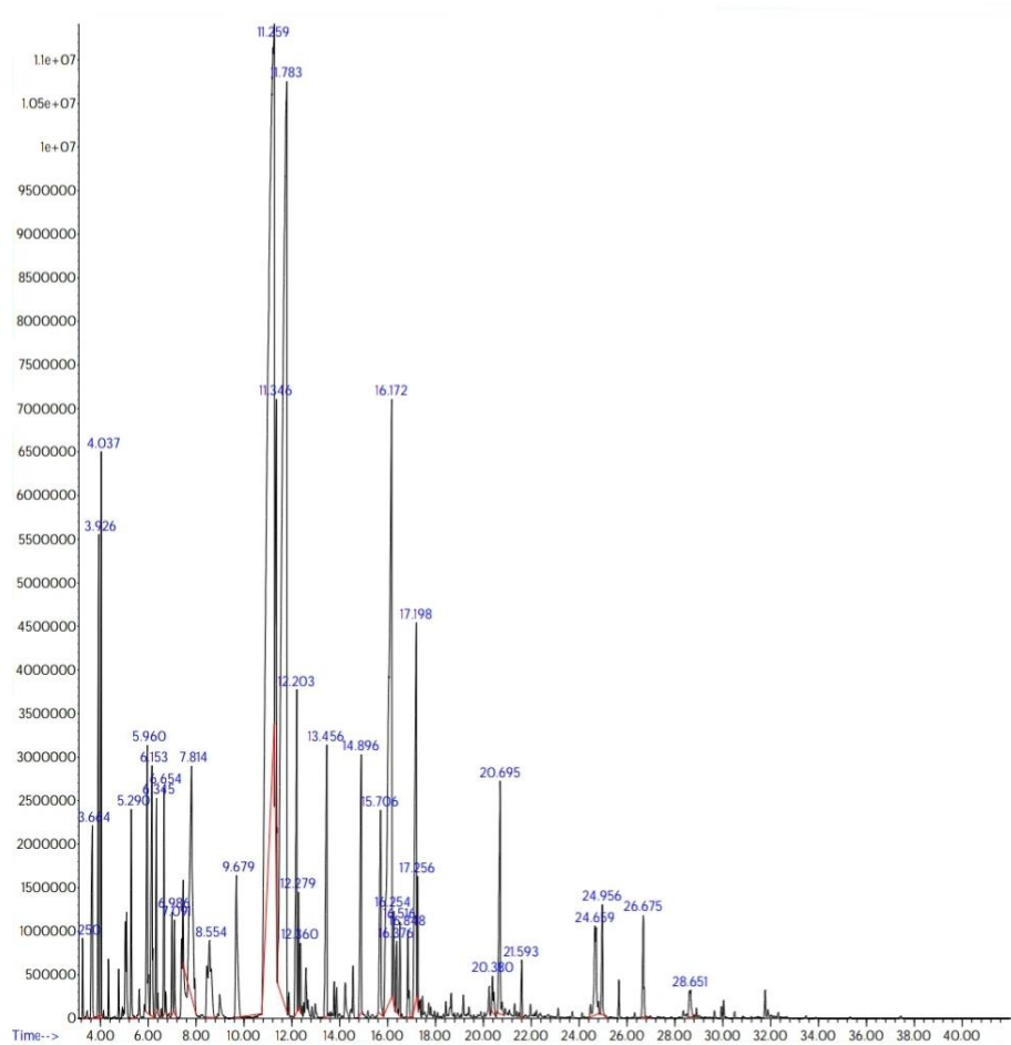
Figure. Heracleum persicum GC/MS chromatogram
