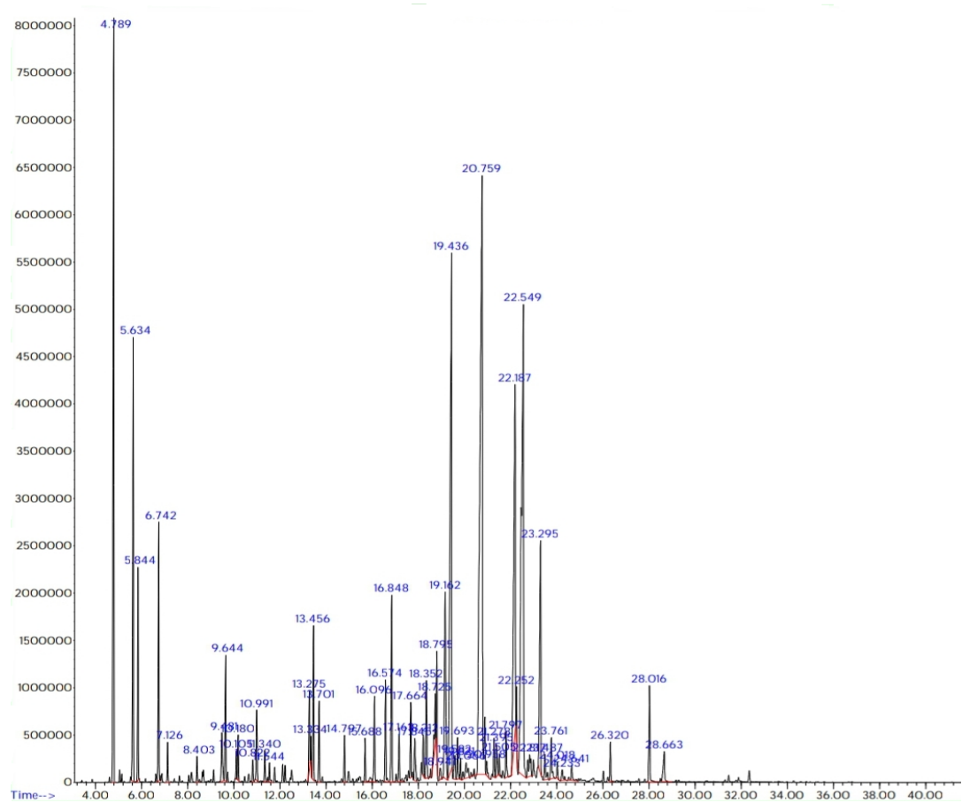
Figure. Teucrium polium GC/MS chromatogram
